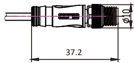
M8 Connector
